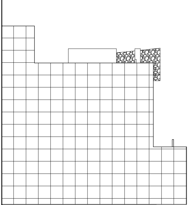
NORTH ELEVATION
