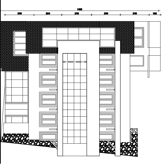
SOUTH ELEVATION
