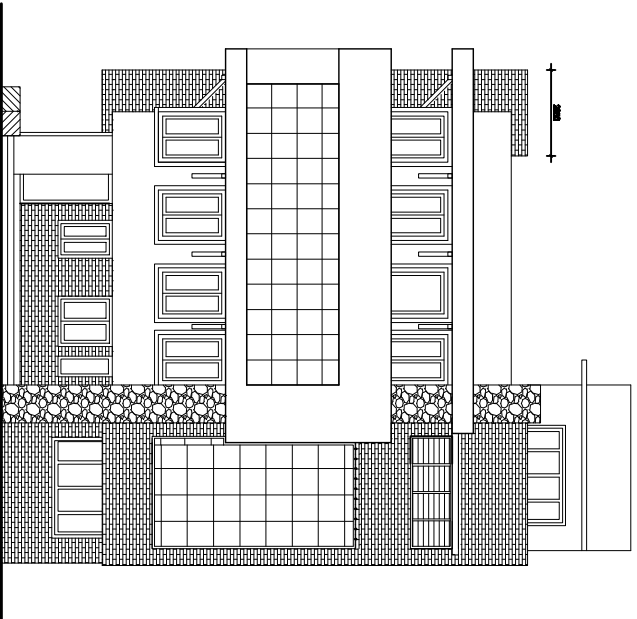
EAST ELEVATION
