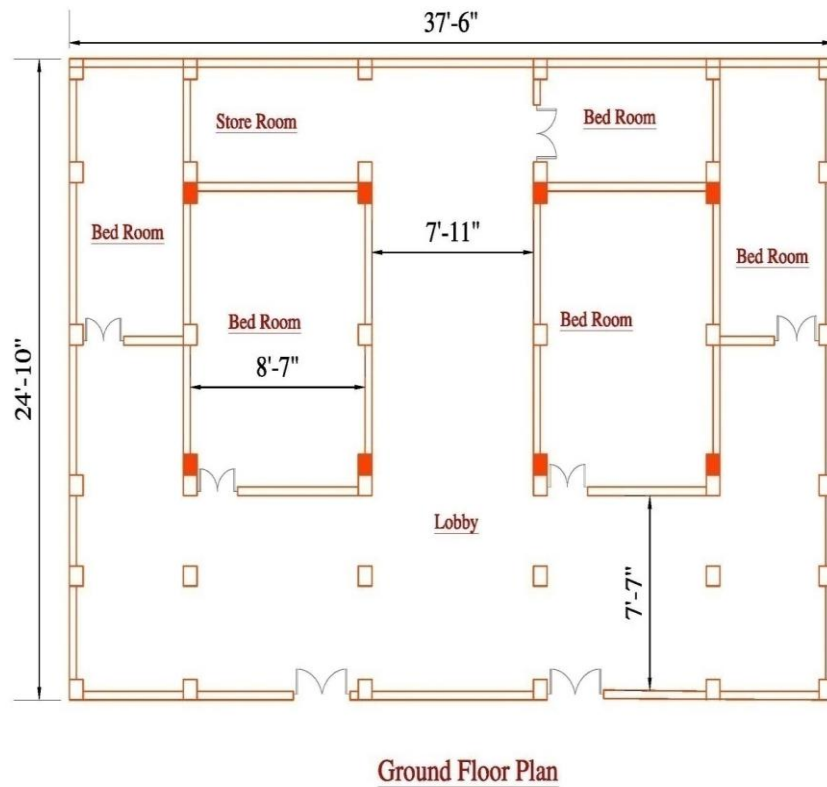
Figure 20. Ground Floor Plan of Dhangadi Residence
